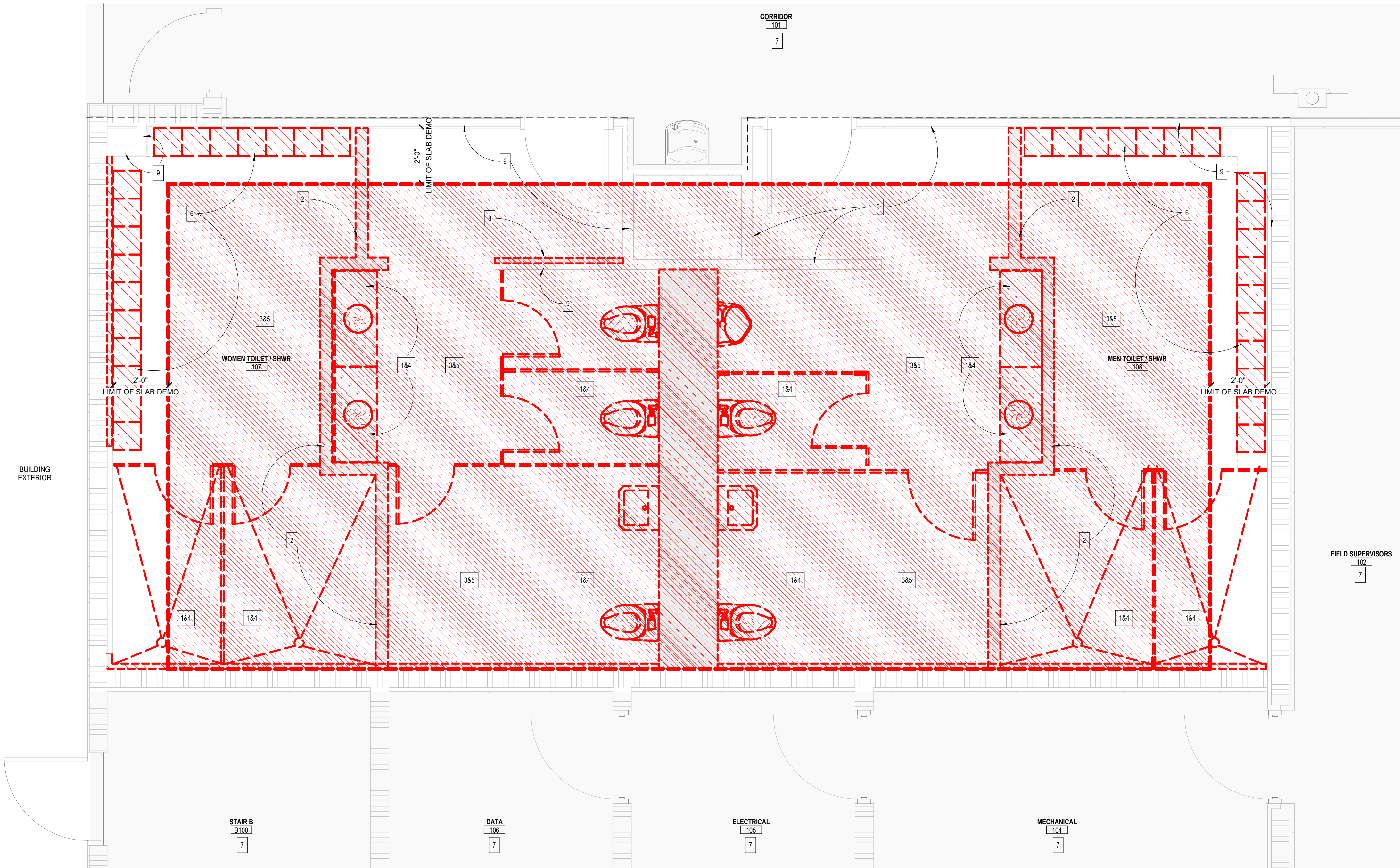
DEMO 1ST FLOOR PLAN
